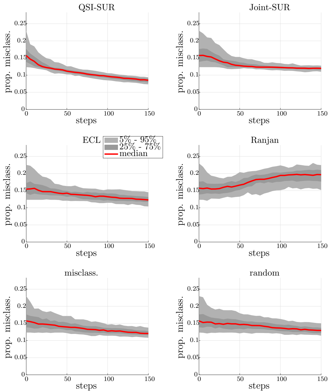
Figure SM6: Median and several quantiles of the proportion of misclassified points vs. number of steps, for 100 repetitions of the algorithms on the test function f_2 .
