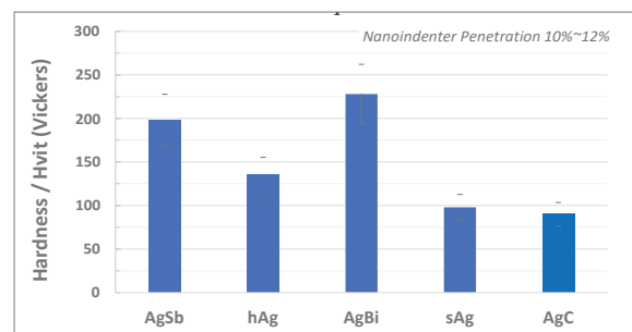
Fig.2 : Hardness (Hvit) measurements, using nanoindentation, on flats electroplated with various silver based deposits
