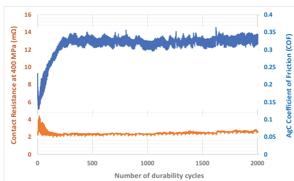
Fig.4.1 : Electrical Contact Resistance and Friction Coefficient evolution of AgC silver-carbon electrodeposit according to durability cycles
