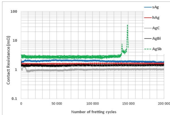
Fig.4.3 : Electrical Contact Resistance evolution of various silver-based deposits according to the number of fretting cycles under 650 MPa of contact pressure
