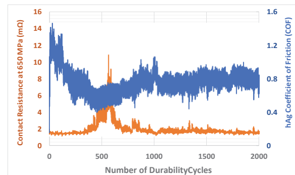
Fig.4.2 : Electrical Contact Resistance and Friction Coefficient evolution of hAg Hard Pure Silver electrodeposit according to durability cycles
