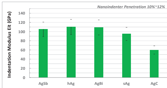
Fig.3 : Indentation modulus measurements, using nanoindentation, of flats electroplated with various silver based deposits
