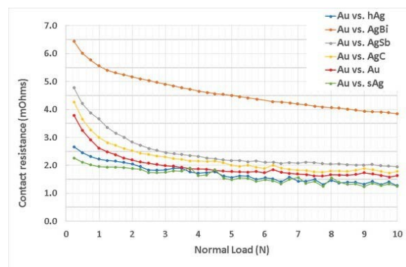
Fig.1 : Contact resistance evolution vs. normal force between between Au/Ni hemispheres & flats plated
