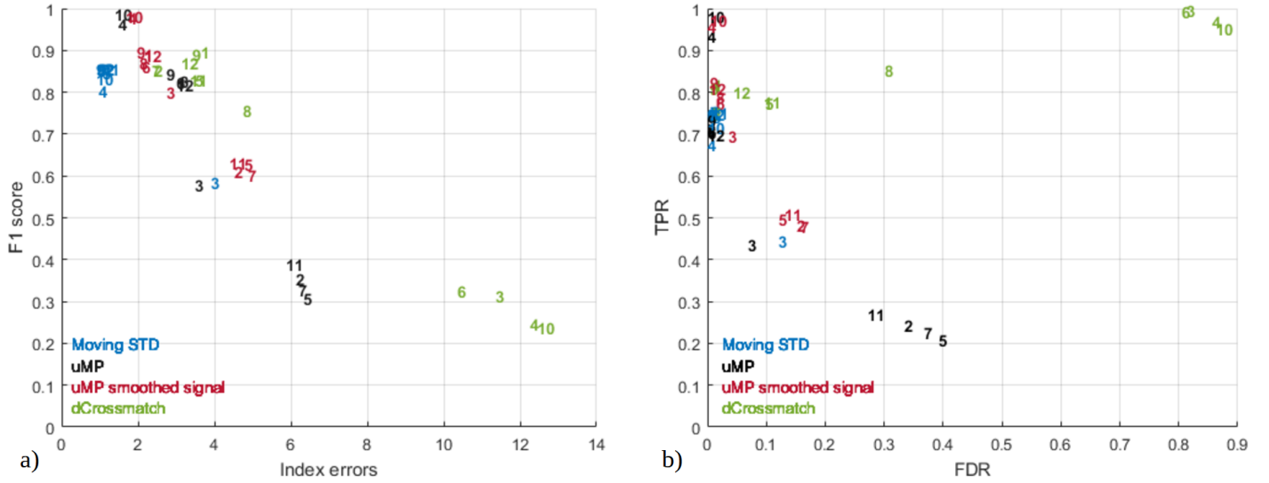
Fig. 6: Visualization of a) the couple of F1-score F_1 and motif location error e , and of b) TPR vs. FDR, for all cases of time series. Each case is represented by a number.
