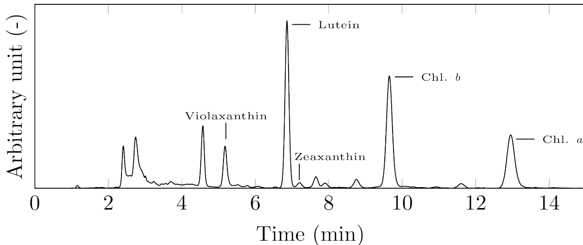
Fig. 1. Chromatogram of a random sample obtained with the method described in Section 3.2
