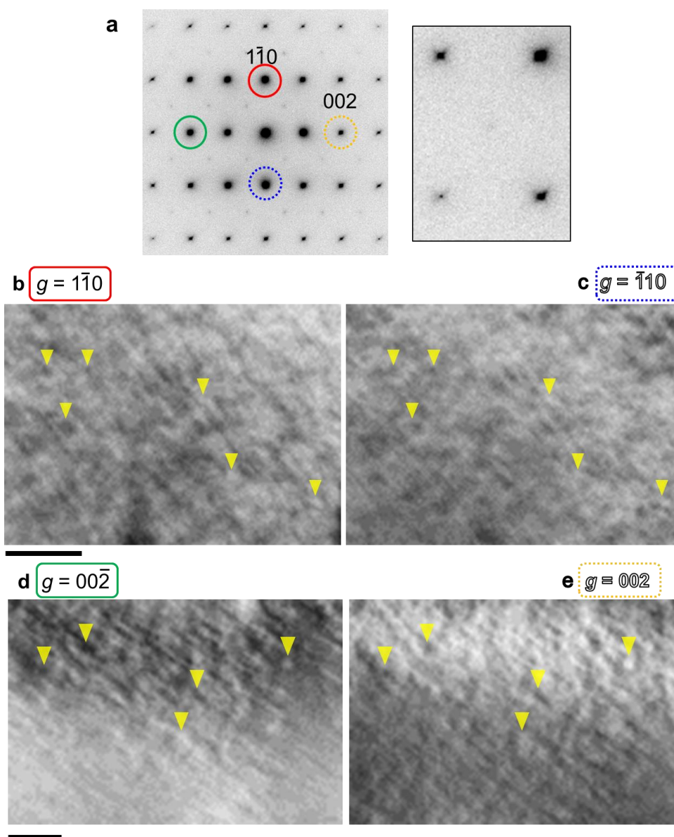
Figure 4 Polar nanoregions in PYN-0.4PT. (a) Electron diffraction pattern along [110] . The right panel is a magnified image. (b, c) [1\bar{1}0] components of the polar nanoregions: Dark-field images based on the (b) 1\bar{1}0 and (c) \bar{1}10 reflections. (d, e) [001] components of the polar nanoregions: Dark-field images based on the (d) 00\bar{2} and (e) 002 reflections. The contrast in images (c) and (e) was reversed by reversing the experimentally obtained intensities. In (b) and (c) and similarly in (d) and (e), the arrowheads point to the sites of equal contrast, which demonstrates the contrast reversal between the dark-field images of the g and \bar{g} reflections. All images were obtained on the same grain. The scale bars are 100 nm.
