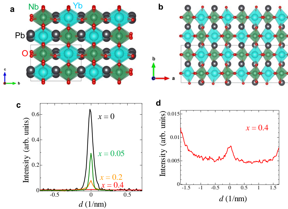
Supplementary Figure 4. \{1/2 1/2 1/2\} cation-ordering structure and composition dependence of the intensities of \{1/2 1/2 1/2\} spots. (a, b) Schematics of the Pmna structure along a and c axes. (c) Intensity profile of the \{1/2 1/2 1/2\} spot in each composition. The intensities of the \{1/2 1/2 1/2\} spots are normalized by those of the 111 reflections in electron diffraction patterns. (d) Magnified profile of x = 0.4 in panel (c).
