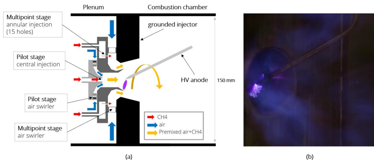
Fig. 2 (a) Schematic of the two-stage injector with the high-voltage electrode. (b) Photograph of the electrode with NRP discharges applied in a 60-kW flame. Credit Auguste & Louise SARL.
