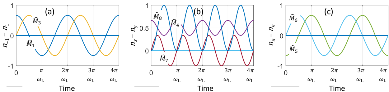
Figure 7. Time evolution of the population difference between states (a) |{-1}\rangle_z and |{1}\rangle_z , (b) |\Psi_x\rangle and |\Psi_y\rangle , and (c) |\Psi_u\rangle and |\Psi_v\rangle for different mechanisms.
