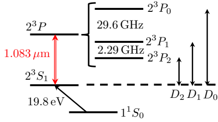
Figure 1. Level structure of {}^4\text{He} . The three transitions D_0 , D_1 , and D_2 from the metastable 2^3S_1 level are well separated, by a difference larger than the 0.8 GHz Doppler broadening at room temperature.
