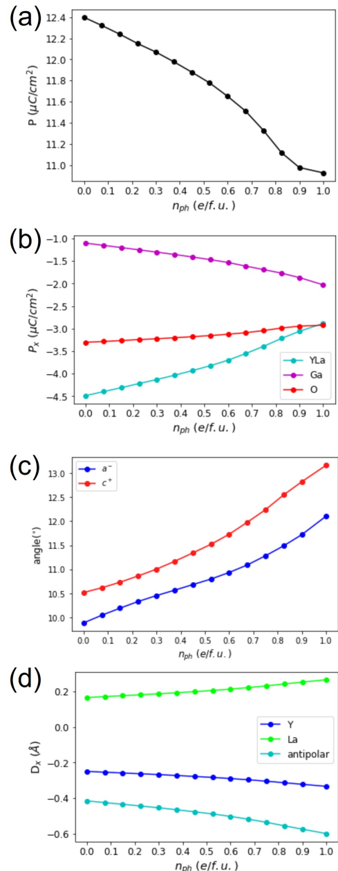
FIG. 2. Variations of different quantities with the number of photo-excited carriers n_{\text{ph}} . (a) Magnitude of polarization P . (b) P_x component contributed by A-site cations La and Y, Ga and oxygens, respectively. (c) The out-of-phase tilting ( a^- ) angle and in-phase tilting ( c^+ ) angle. (d) The in-plane ionic displacement D_x^{\text{Y}} , D_x^{\text{La}} , and antipolar displacement D_x^{\text{Y}} - D_x^{\text{La}} .
