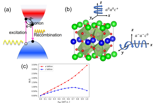
FIG. 1. (a) Three dynamic events electrons experience after illumination, including photo-excitation, electron-electron/electron-phonon interaction, and electron-hole recombination. (b) Illustration about out-of-plane, in-phase tilting c^+ and in-plane, out-of-phase tilting a^- in \text{LaGaO}_3/\text{YGaO}_3 . Two arrows indicate tilting directions of octahedra in front and rear layers around respective axis, respectively. (c) Photo-induced strain for in-plane a and out-of-plane c lattice constants as a function of photo-excited carriers n_{ph} .
