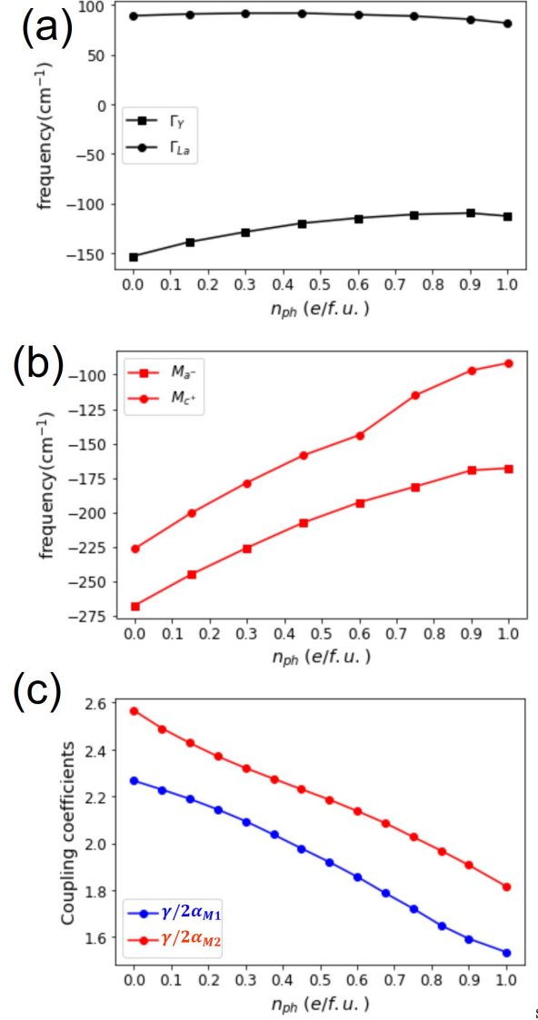
FIG. 3. Changes of phonon frequencies with n_{\text{ph}} in the parent tetragonal cell. (a) The Y-dominant and La-dominant antipolar modes at zone-center \Gamma -point (0, 0, 0) . (b) Modes at zone-boundary M-point (1/2, 1/2, 0) denoting a^- and c^+ tiltings. (c) Changes of trilinear coupling coefficients \gamma/2\alpha_{M_{1,2}} with n_{\text{ph}} in the parent tetragonal cell.
