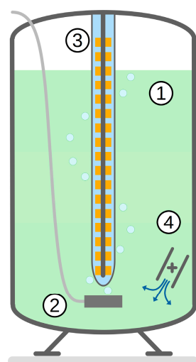
Figure 1. Schematic of the photobioreactor used for the study. 1—culture medium, 2—air sparger, 3—LED light source, 4—circulating pump.
