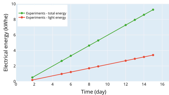
Figure 4. Total process consumed electrical energy and light consumed electrical energy over time. Measurements started after 24 h. Fitted values: total energy (kWh) = 0.662 \times \text{time (day)} \pm 0.000 . R^2 = 1 . Lighting energy (kWh) = 0.244 \times \text{time (day)} \pm 0.000 . R^2 = 1 .
