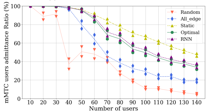
(c) Admittance ratio of mMTC users
