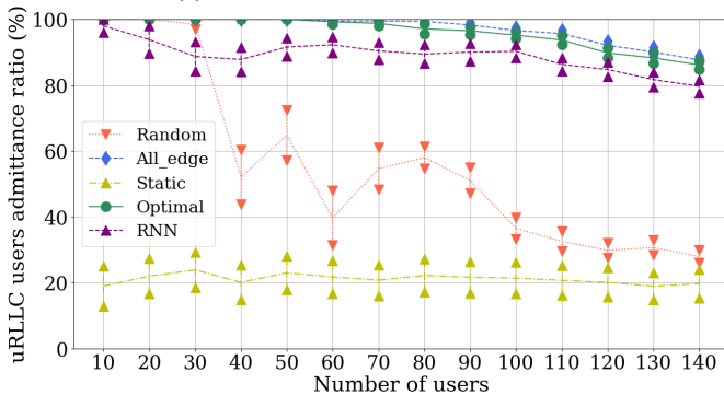
(b) Admittance ratio of uRLLC users
