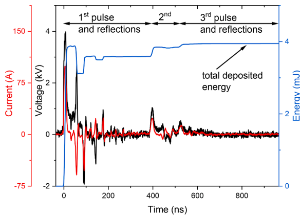
Fig. 3. Typical voltage, current, and energy traces measured during the experiments.
