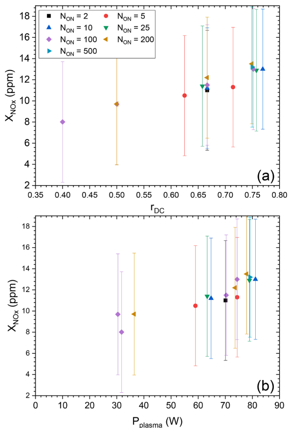
Fig. 15. Evolution of the NO x concentration at the chamber outlet for various pulse patterns of NRP discharges applied in a 50-kW flame at \Phi_g = 0.44 and \alpha = 40\% as a function of (a) the duty cycle ratio and (b) the average plasma electric power.
