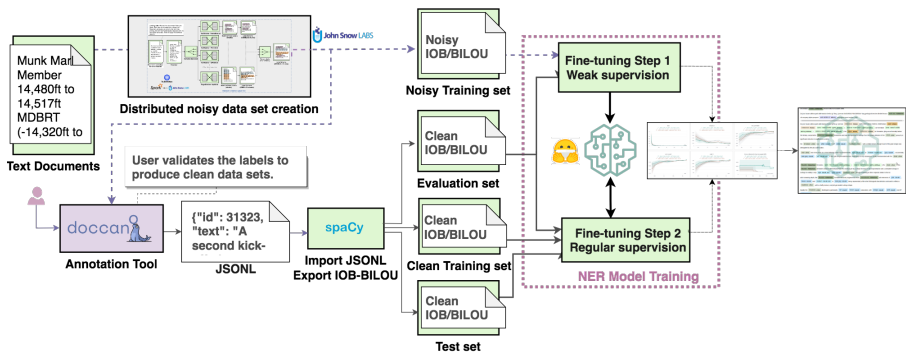
Fig. 2 Implementation pipeline.
