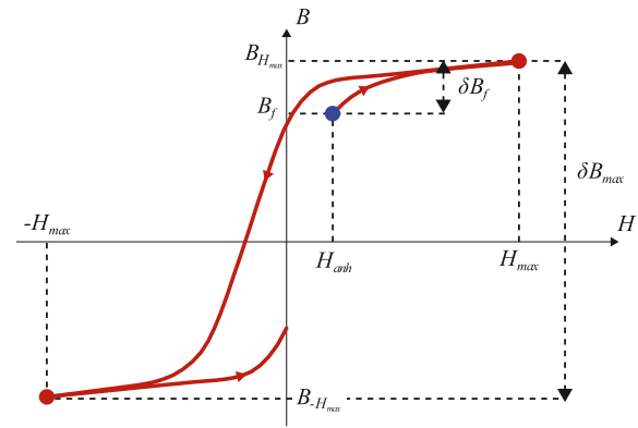
Fig. 18. Major loop obtained after the anhysteretic measurement procedure for an accurate evaluation of the anhysteretic magnetic field B_{anh} . The blue point is the final point of the anhysteretic procedure (Fig. 17) and the red line is the final loading to obtain B_{anh} . (For interpretation of the references to color in this figure legend, the reader is referred to the web version of this article.)
