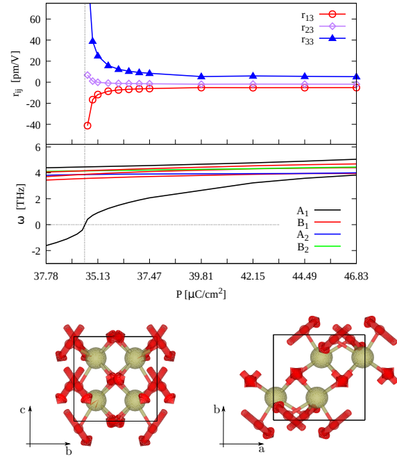
FIG. 4. Top The top panel reports the r_{13}, r_{23}, r_{33} coefficients as a function of the polarization P for HfO 2 . The bottom panel report the lowest phonon frequencies at \Gamma as a function of P . The softening mode is represented in black. Bottom , two views of the atomic displacements corresponding to the softening mode are reported. The Hf atoms are represented in gold, the oxygen atoms in red. The arrows represent the atomic displacements.
