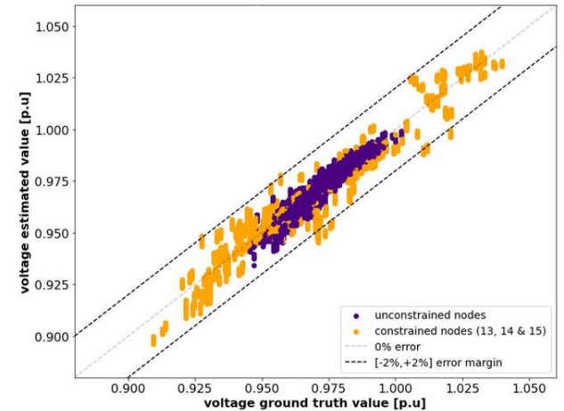
Figure 7. Voltage estimation scatter
