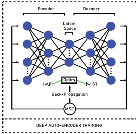
Figure 1. Auto-encoder training
