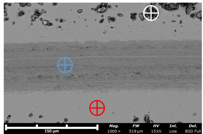
Fig. 8. Observation of the wear track of the disc after 50 000 laps with a SEM in BSD mode – x1000 – Locations of EDX analysis: light grey area corresponds to the unworn area (red cursor); dark grey area corresponds to the wear track (blue cursor); white cursor highlights the wear debris around the wear track
