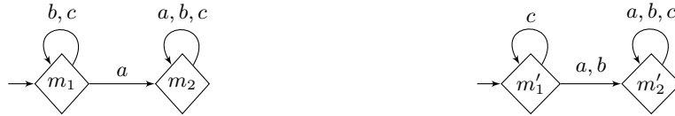
■ Figure 1 Memory skeletons \mathcal{M} (left) and \mathcal{M}' (right) for two-target reachability games. In figures, diamonds (resp. circles, squares) represent memory or automaton states (resp. arena vertices controlled by \mathcal{P}_1 , arena vertices controlled by \mathcal{P}_2 ).
