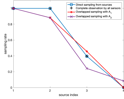
Figure 6. Impact of overlapped source observation ( N = 4 , R = 40 RBs, \text{CQI}=[10, 8, 6, 4] ).
