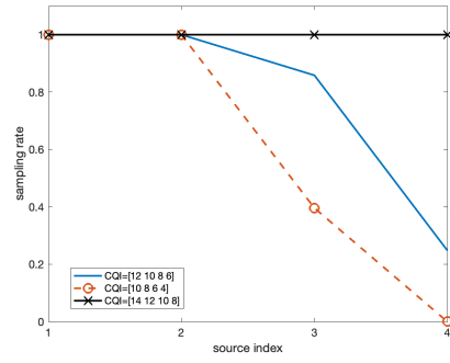
Figure 4. Impact of different channel conditions ( N = 4 , R = 40 RBs).
