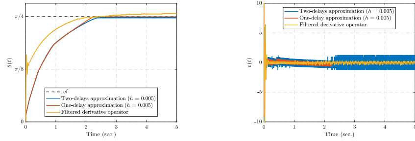
(a) Plant output when in closed-loop with the controllers C_0 implemented with a filter, C_1 and C_2 .
