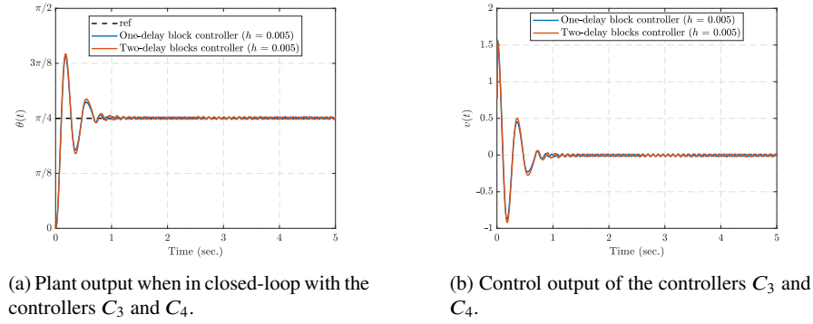
Fig. 4: Real plant output considering the different proposed controllers.
