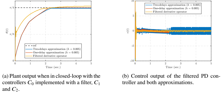
Fig. 3: System output considering the different proposed controllers.
