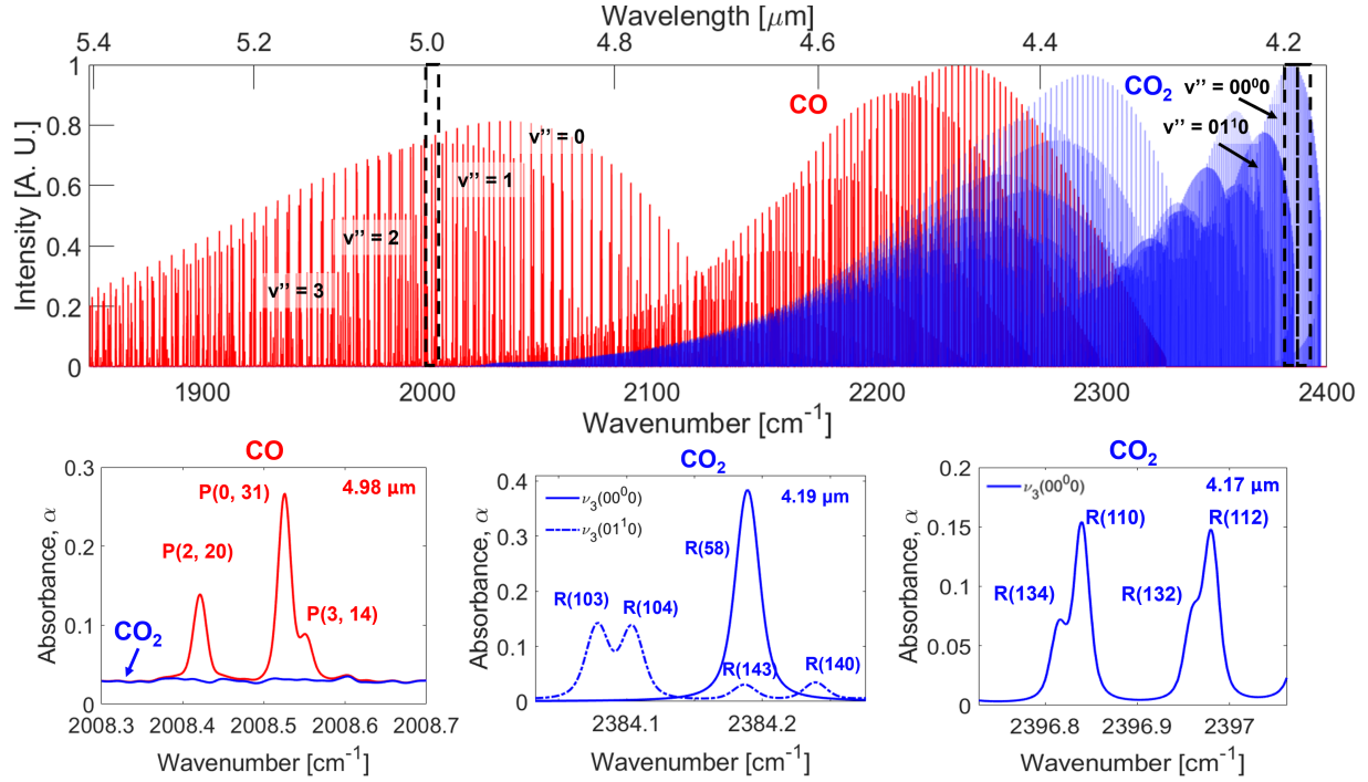
Fig. 2 Line survey of the fundamental bands of CO and the asymmetric stretch fundamental bands of CO 2 from 4.2 - 5.4 \mu\text{m} (top) Simulated spectrum of resolved transitions of CO (bottom left), and CO 2 (bottom middle and bottom right) using the HITEMP database [27]. Vibrational lower state of CO 2 is denoted with the solid/dashed lines at 4.19 and 4.17 \mu\text{m} . CO 2 absorption at 4.98 \mu\text{m} is from many different vibrational bands and the CDSD database [29] was used at this wavelength. Spectra are simulated at 3300 K, 0.3 atm, 10.16 cm optical pathlength, 0.1 mole fraction of CO 2 , and 0.02 mole fraction of CO. At 4.98 \mu\text{m} , the CO spectrum (bottom left) is presented as a sum with the CO 2 baseline.
