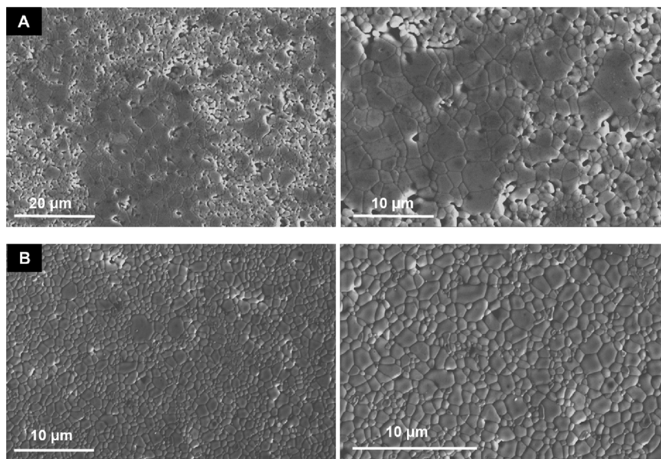
Fig. 1 – SEM micrographs of the sintered Y_2SiO_5 ceramics: (a) conventionally sintered Y_2SiO_5 , (b) spark-plasma sintered Y_2SiO_5 .
