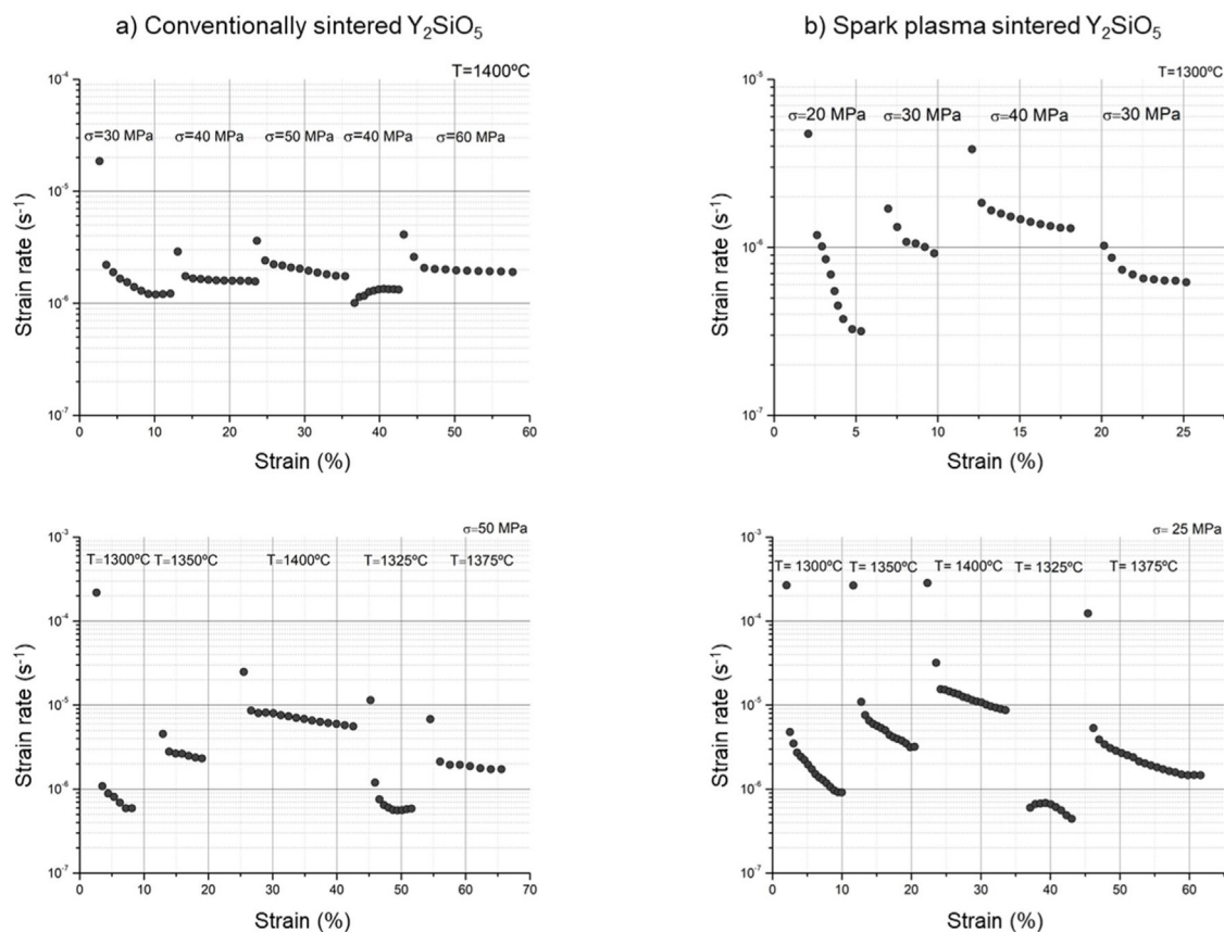
Fig. 6 – Strain rate vs. strain curves for: (a) conventionally sintered Y_2SiO_5 in constant temperature (top) and constant stress (bottom) tests, (b) spark-plasma sintered Y_2SiO_5 in constant temperature (top) and constant stress (bottom) tests.
