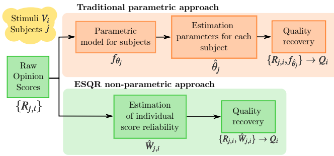
Fig. 1. Parametric approaches assume that the observed opinion scores come from a probabilistic model f_{\theta} , that depends on a finite set of parameters \theta . The parameters \theta are then estimated, and the subjective quality Q is recovered from the assumed probabilistic model using the estimated parameters. The proposed non-parametric approach (ESQR) instead measures how reliable is each single opinion score without resorting to a predefined model. The recovered quality Q is then computed as a weighted sum of the opinion scores in which the weight of each opinion score is determined by its reliability.
