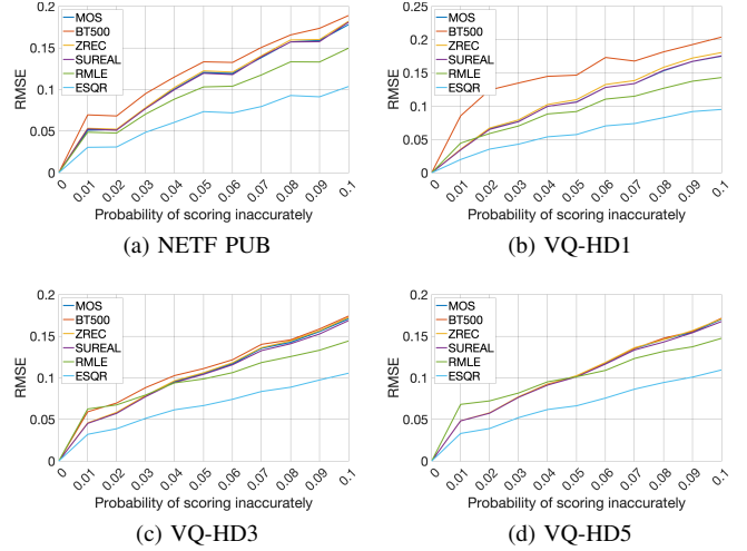
Fig. 2. Robustness to noise insertion. RMSE between the quality recovered on the original dataset and under different noisy conditions. The noise was added by replacing a given fraction of the opinion scores (see the x -axis) of each subject with integer numbers sampled at random between 1 and 5. The simulation was run with 30 different seeds and the curve for each quality recovery method reports the average RMSE from the 30 trials.
