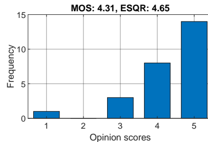
Fig. 7. Quality estimates of ESQR vs. other methods. Opinion scores distribution for a stimulus with high discrepancy between Q (ESQR) and the mean opinion score (MOS).
