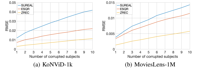
Fig. 5. Crowdsourcing experiments, robustness to spammer annotators. Comparing the robustness of the ESQR algorithm, the Netflix SUREAL software and ZREC to the insertion of spammer annotators on two crowdsourcing datasets. A certain number of spammer annotators (see the x-axis) was added to each dataset. The opinion scores of a spammer annotators are integers sampled at random between 1 and 5. The RMSE between the quality recovered on the original dataset and the one obtained after adding spammer annotators is reported on the y-axis.
