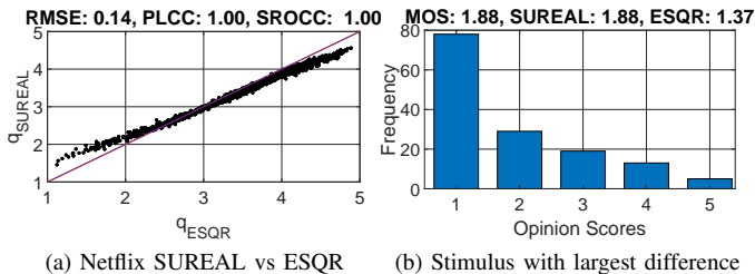
Fig. 8. Quality estimates of ESQR vs. other methods. Comparing the output of the ESQR algorithm to the one of the Netflix SUREAL software on the MovieLens-1M dataset. On the right, the distribution of opinion scores of the stimulus for which the outputs of the two approaches differ the most.
