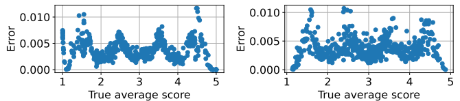
(a) Normal. Average L1 error is 0.004. (b) Beta. Average L1 error is 0.004.
