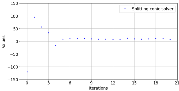
(a) Splitting conic solver
