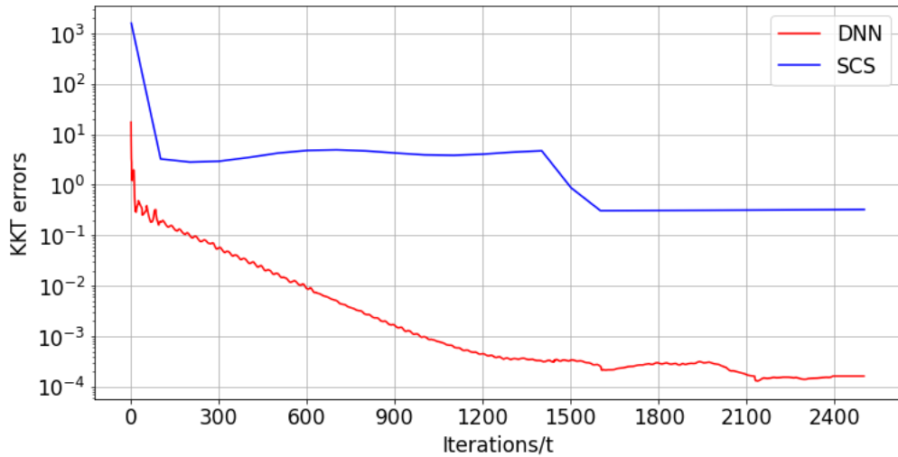
Figure 3: Comparison of the convergence of DNN and SCS methods. The instance is with game size 10 * 10 . The x-axis represents the number of iterations (SCS method) or time (DNN method). The y-axis represents the \epsilon error for the KKT conditions.
