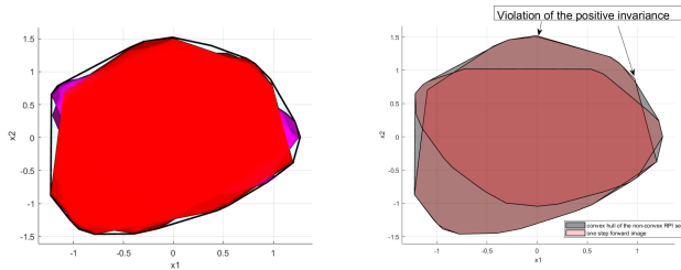
Fig. 2. (Left) approximation of the mRPI set X_\infty , the union of red and magenta sets, compared with the convex RPI obtained above. (Right) Illustration of the violation of positive invariance for \text{co}(X_\infty) .
