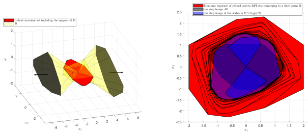
Fig. 1. (Left) RPI set (red) constructed using (11) where Z_0 = \text{supp}(\mathcal{D}_1) . (Right) Iterative RPI refinement converging to a tight convex RPI set.
