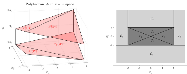
Fig. 5. Left: Polytope \mathcal{W} in the x-w space, with \mathcal{F}_i^2(\mathcal{W}) in red satisfying Theorem 2i). Right: the corresponding partition in \mathbb{R}^2 .
