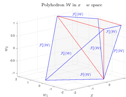
Fig. 1. Set \mathcal{W} (1) for Example 1, with \mathcal{F}_i^n(\mathcal{W}) in blue and red satisfying Theorem 2(i) and Theorem 2(ii), respectively.
