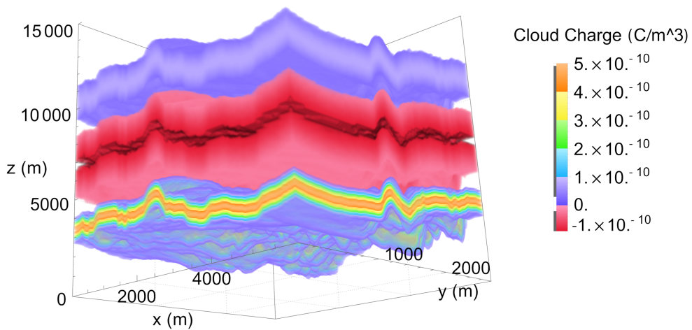
Figure 4. Cloud structure modelling: red negative space charge, blue to orange positive space charge.
