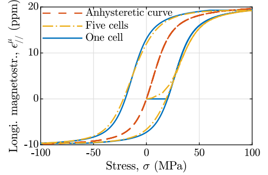
Fig. 5. Impact of a discrete distribution of pinning stresses on the strain-stress curve. Equivalent single-crystal isotropic material with parameters: M_s = 1.71 MA/m, \lambda_s = 21 ppm, K_1 = K_2 = 0 . One cell parameters: \kappa_{\sigma} = 20 MPa, \omega = 1 . Five cell parameters: \kappa_{\sigma} = [0; 5; 15; 22; 26; 34] MPa, \omega^k = [0.05; 0.1; 0.25; 0.25; 0.2; 0.15] .
