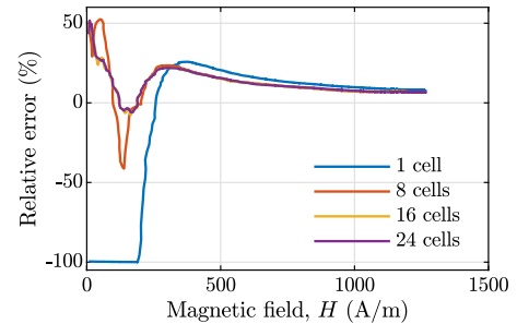
Fig. 25. Relative error between measurements and model.
