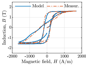
(b) Comparison of measured and modeled induction as a function of magnetic field
