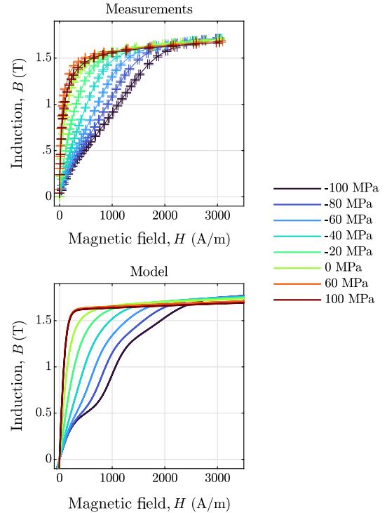
Fig. 18. Comparison between measured [30] and modeled anhysteretic magnetic behavior under several levels of static uniaxial stress.
