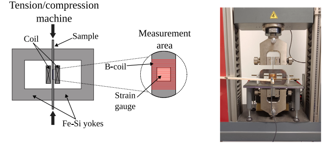
Fig. 8. Magneto-mechanical setup.
