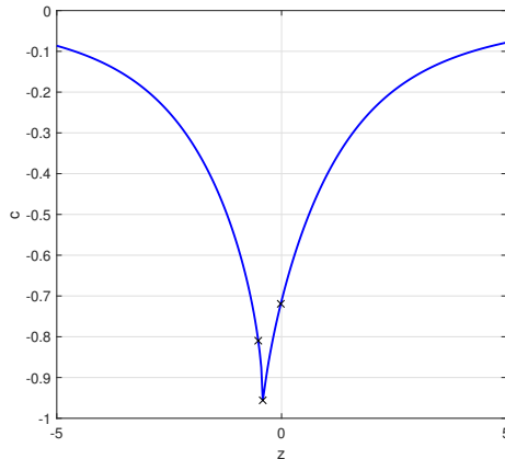
Fig. 6 Minimum spectral abscissa c as a function of plant parameter z , for p = -10 . The values of the zeros, indicated with crosses, refer to the experiments reported in Figure 7 and the accompanying text.
