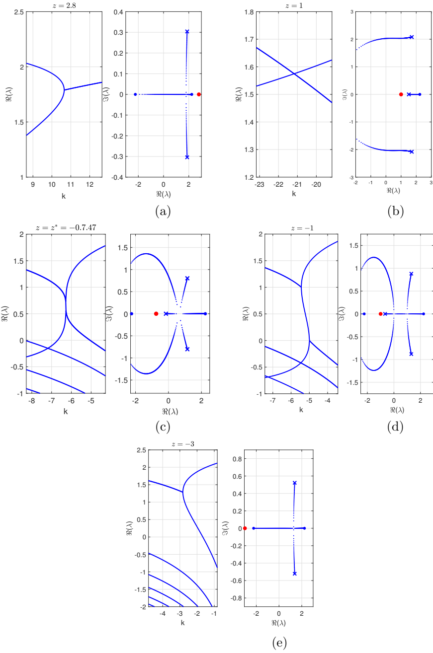
Fig. 5 Real parts of the rightmost characteristic roots as a function of controller parameter k and associated root locus around the global minimum, for p = 5 and different values of z , indicated in Figure 4. In the root locus, the branches go from the blue dots to the blue crosses for increasing |k| . The red dot indicates the plant's zero location.
