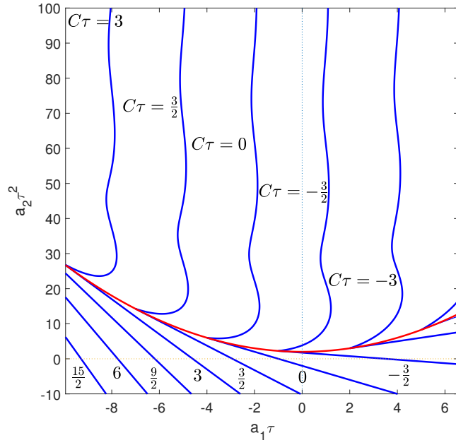
Fig. 2 Level sets of the global minimum of the spectral abscissa of (1)-(2) and (4) in the plant-parameter space (a_1, a_2, \tau) . The level is indicated with the value of C\tau .
