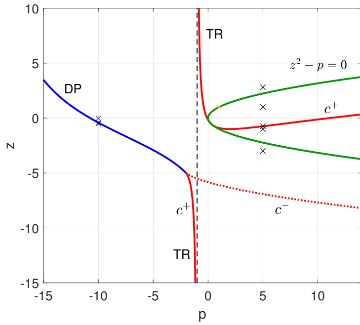
Fig. 3 Curves corresponding to configurations DP, TR and a pole-zero cancellation in the (normalized) plant parameter space (p, z) . The plant parameters indicated with crosses refer to the experiments reported in Figures 5 and 7 and the accompanying text.
