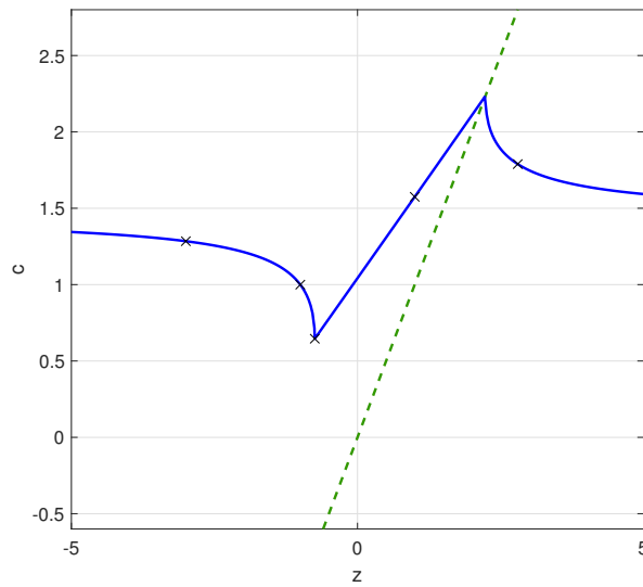
Fig. 4 Minimum spectral abscisa c as a function of plant parameter z , for p = 5 . The dashed line is described by c = z . The values of the zeros, indicated with crosses, refer to the experiments reported in Figure 5 and the accompanying text.
