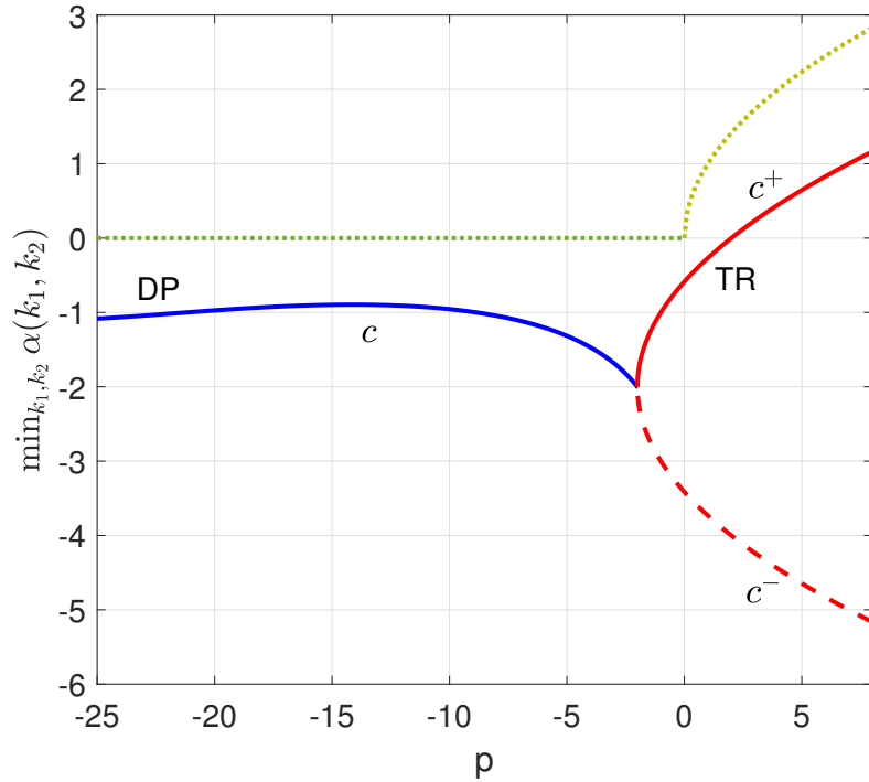
Fig. 1 Global minimum of the spectral abscissa (11) as a function of (normalized) plant parameter p . The segment to the left of p = -2 relates to a complex conjugate pair of rightmost characteristic roots with multiplicity two, the two branches to the right to the presence of a real root of multiplicity three. The top branch corresponds to a rightmost root and global minimizer of the spectral abscissa function. The dotted segments depict the spectral abscissa of the open loop system.
