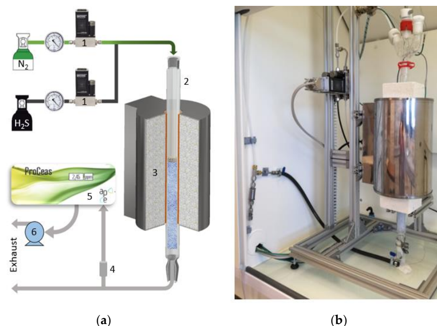
Figure 1. (a) Schematic view; (b) and picture of the experimental setup used for the sulfidation tests. 1—mass flow meter, Brooks Instrument; 2—glass reactor with an internal diameter of 3 cm; 3—tube furnace; 4—sampling nozzle providing a flow rate of about 3 L/h through the AP2E analyzer; 5—AP2E analyzer; 6—AP2E analyzer pump.
