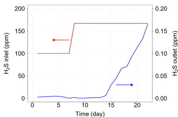
Figure 2. Breakthrough curve for 0.8 cm height Hi-Fuel sorbent at 300^\circ\text{C} with the injection of 100 ppm \text{H}_2\text{S} for 7 days followed by 167 ppm \text{H}_2\text{S} for 15 days. Gas flow of mixture \text{H}_2\text{S}/\text{N}_2 — 60\text{ NmL}/\text{min} ( \text{GHSV} = 637\text{ h}^{-1} ).
