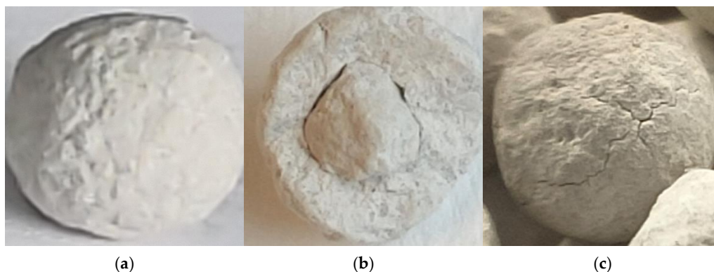
Figure 4. (a,b) Pictures of fresh Hi-Fuel A310 sorbent; (c) converted sorbent.
