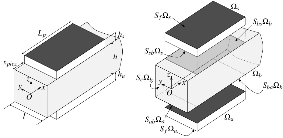
(b) Dimensions of the piezoelectric patches: h = 1.56 \text{ mm} , h_s = h_a = 0.4 \text{ mm} , L_p = 20 \text{ mm} , l = 10 \text{ mm} , x_{piez} = 1 \text{ mm} . (c) Exploded view. The body \Omega_a is the piezoelectric actuator; The body \Omega_s is the piezoelectric sensor; The body \Omega_b is the aluminum beam;
