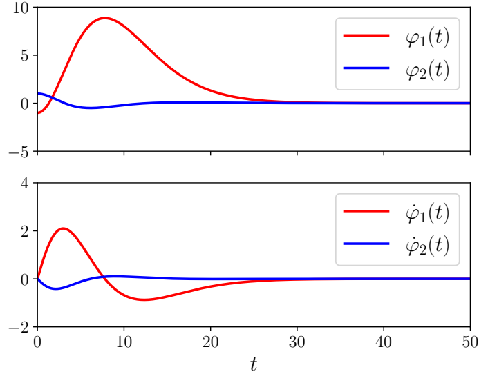
FIGURE 4. The solution of the closed-loop system (61) with (72)-(73) if \tau = 1/2 , p_1 = 2 , p_2 = 1 , and the parameters K_{p,1} , K_{p,2} , K_{d,1} , and K_{d,2} are chosen according to (56) and (75). The initial conditions are taken such that for all t \in [-\tau, 0] one has \varphi_1(t) = -1 and \varphi_2(t) = 1 . The components \varphi_1 and \varphi_2 of the solution \mathbf{q} are shown along with their derivatives.
