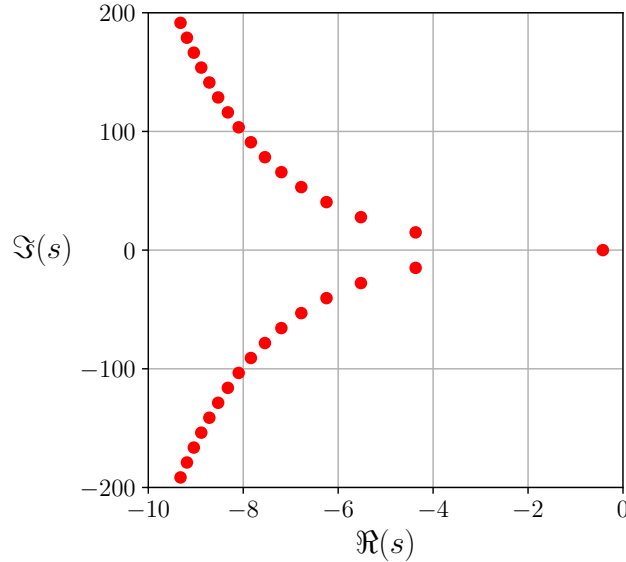
FIGURE 3. The spectrum distribution of the closed-loop characteristic function D in (74) if \tau = 1/2 , p_1 = 2 , p_2 = 1 , and the control parameters b_0 , b_1 , b_2 , and b_3 are chosen according to (56). The spectral abscissa is achieved at the quintuple root s \approx -0.424 . Note that \tau is smaller than \tau_0(2; 1) \approx 0.868 given by (78).
