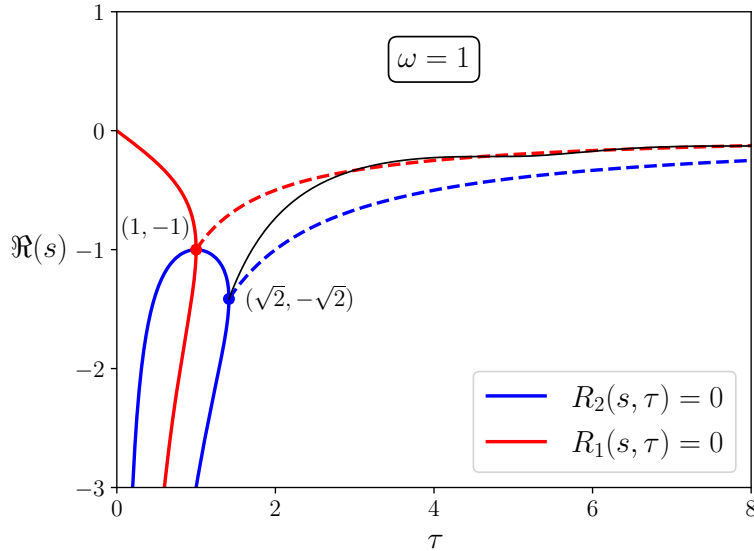
FIGURE 5. Location of the roots of R_1(\cdot, \tau) and R_2(\cdot, \tau) in (82)-(83) and the minimum of the spectral abscissa of D in (81) with respect to b_0 and b_1 for \omega = 1 and \tau > 0 . Solid blue and red lines: real roots of R_2(\cdot, \tau) and R_1(\cdot, \tau) ; dashed blue and red lines: real parts of the non-real roots of R_2(\cdot, \tau) and R_1(\cdot, \tau) ; solid black line: the minimum of the spectral abscissa of D for \tau > \sqrt{2} . For 0 < \tau \leq \sqrt{2} , the minimum of the spectral abscissa of D coincides with the largest real root of R_2(\cdot, \tau) .
