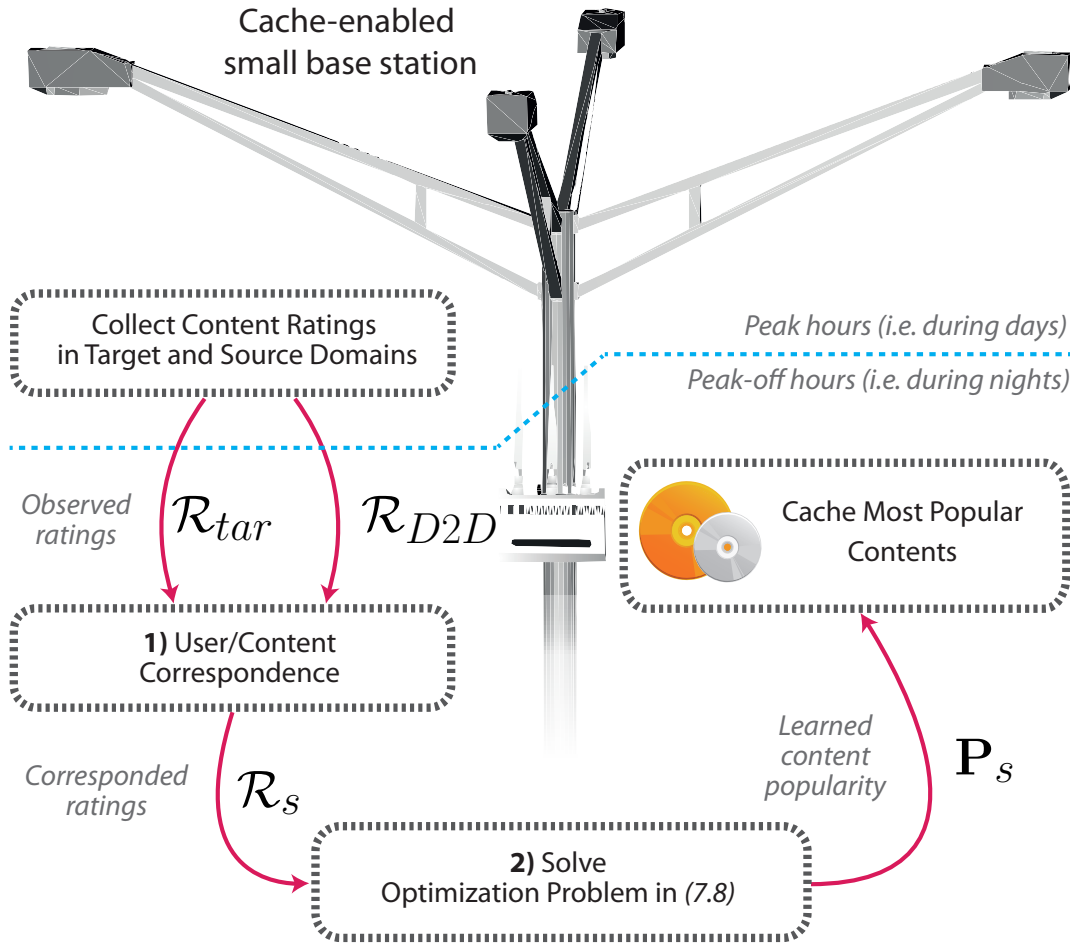
Figure 7.2: An illustration of the proposed TL-based caching procedure.
