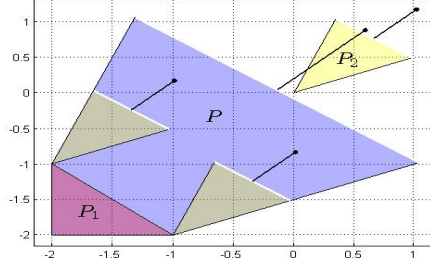
(b) Decomposition of P into the Minkowski sum of P_1, P_2 .
