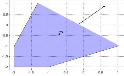
(a) Polyhedron P .
