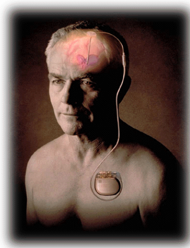
Figure 4.4: Deep-brain stimulation
