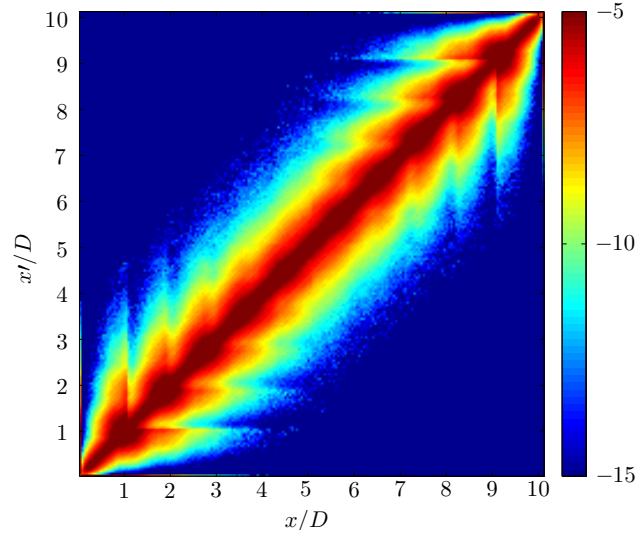
FIGURE 4.7 – Typical example of \ln(\mathcal{P}_I^{e,a}) matrix; \mathcal{N} = 5.10^5 realizations per cell; N_C = 200 , L = 10D , \omega = 0 and \varepsilon_w = 1 .
