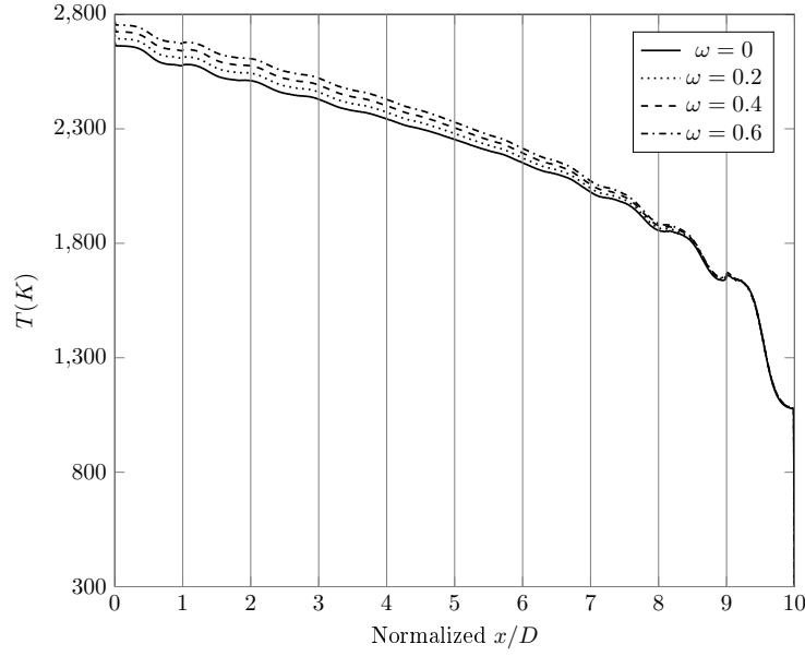
FIGURE 4.13 – Temperature profiles in a scattering and absorbing medium bounded by walls ( \varepsilon_w = 0.4 ) issued from the Monte Carlo approach for \varphi_w = 50 \text{ kWm}^{-2} for various albedo \omega .
