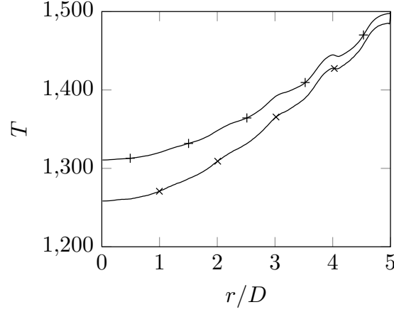
FIGURE 5.7 – Temperature profiles within a purely absorbing medium ( \omega = 0, \varepsilon = 1 : +) and within a scattering and absorbing medium ( \omega = 0.6, \varepsilon = 0.6 : \times ); T_0 = 1500 , and \chi = 4/DkWm^{-3} (or \Phi/2\pi R_t H = 10kWm^{-2} ), N_C = 200 , R_t = 5D
