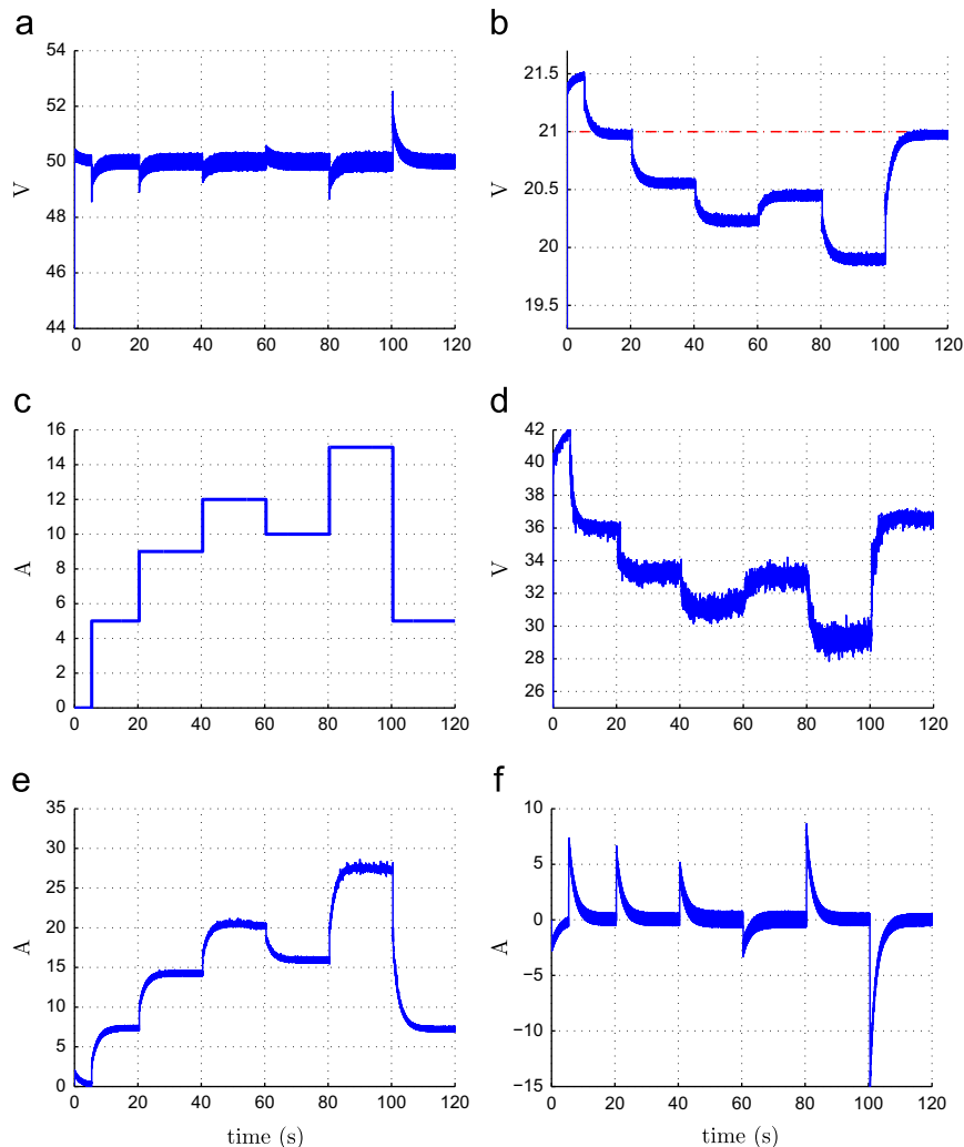
Fig. 10. Experimental result during a step load without an integral action or a load estimator ( \alpha=10, \gamma=0 ). (a) Bus voltage v_b . (b) SCs voltage v_{sc} . (c) Load current i_l . (d) Fuel cell voltage v_{fc} . (e) Fuel cell current i_{fc} . (f) SCs current i_{sc} .
