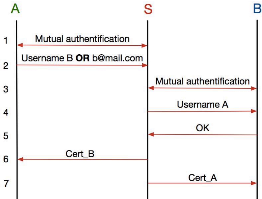
Figure 6.2: Certificates exchange
