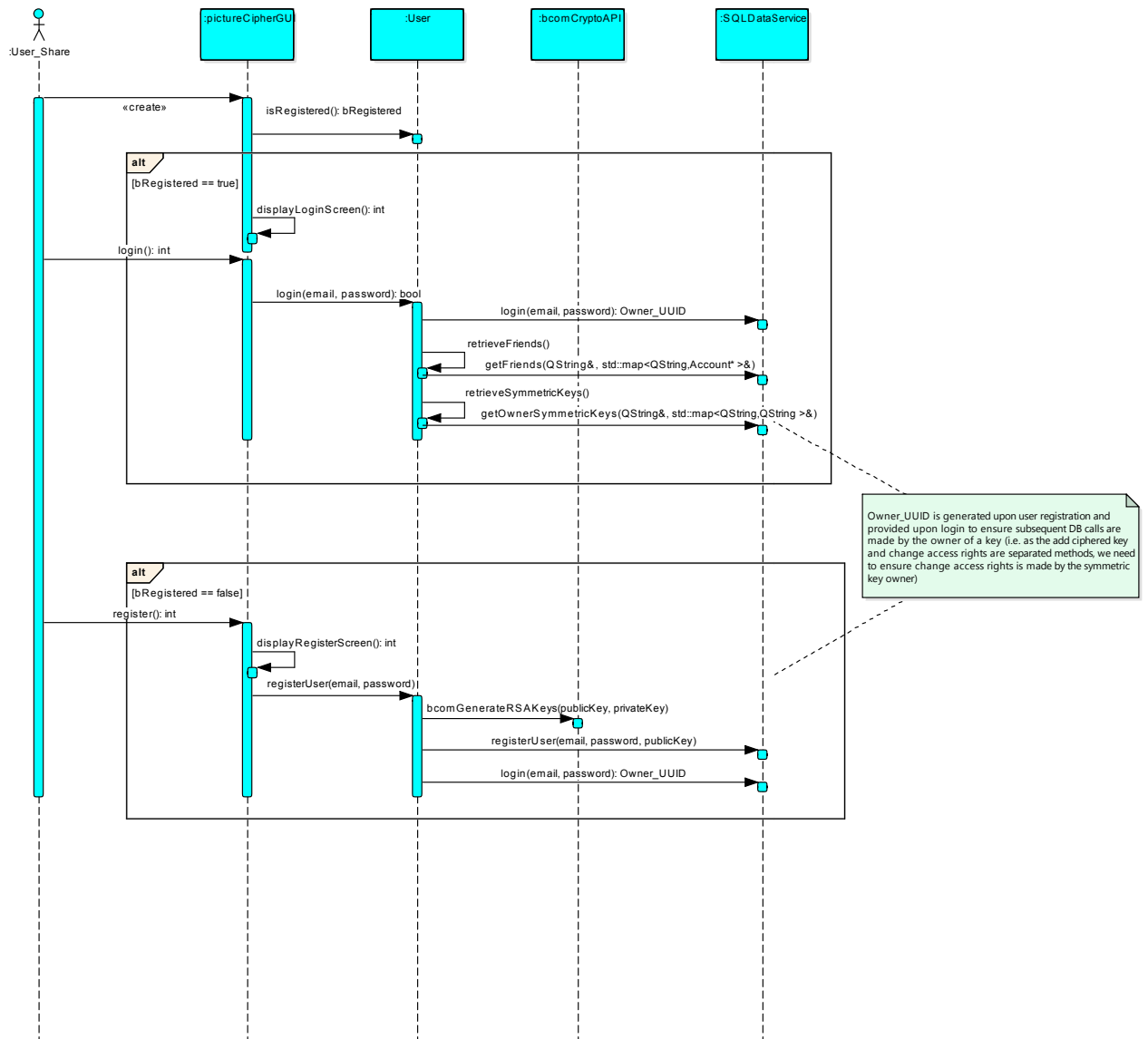
Figure 6.10: The registration in our server
