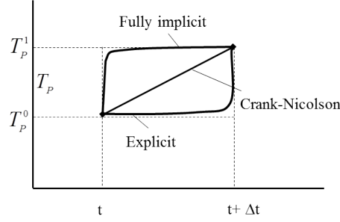
Figure 3.8: Variation of temperature with time for three different schemes
