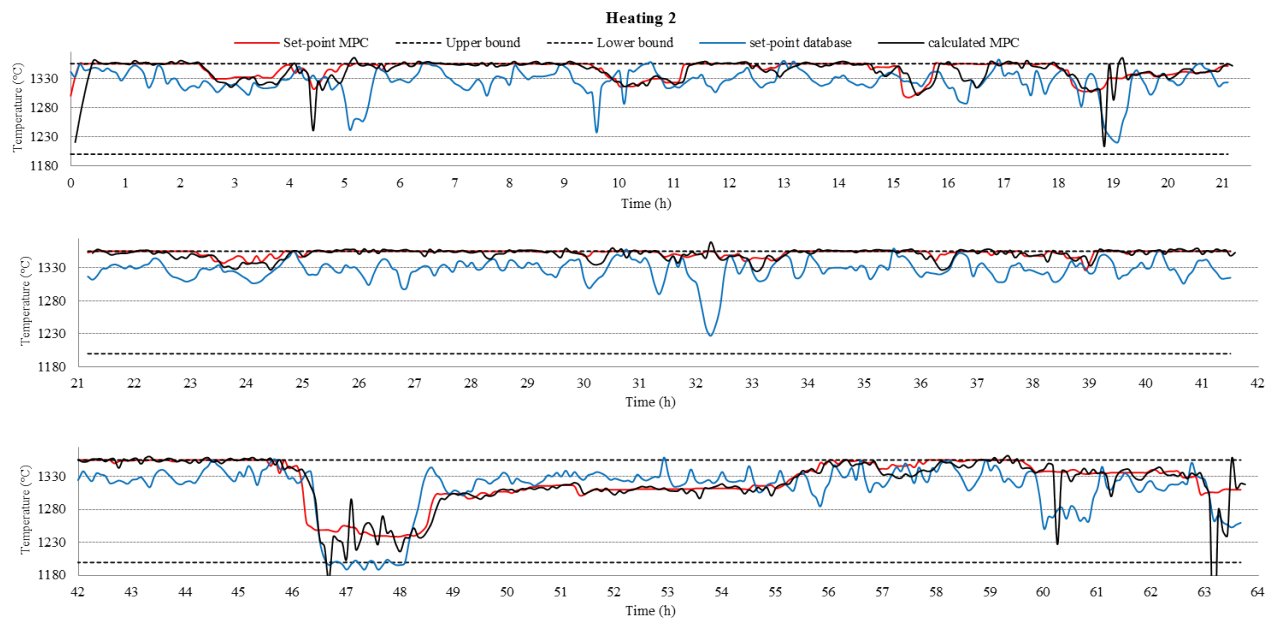
Figure 6.39: Temperature set-point of zone heating 2 calculated by MPC controller compared to that of the existing controller
