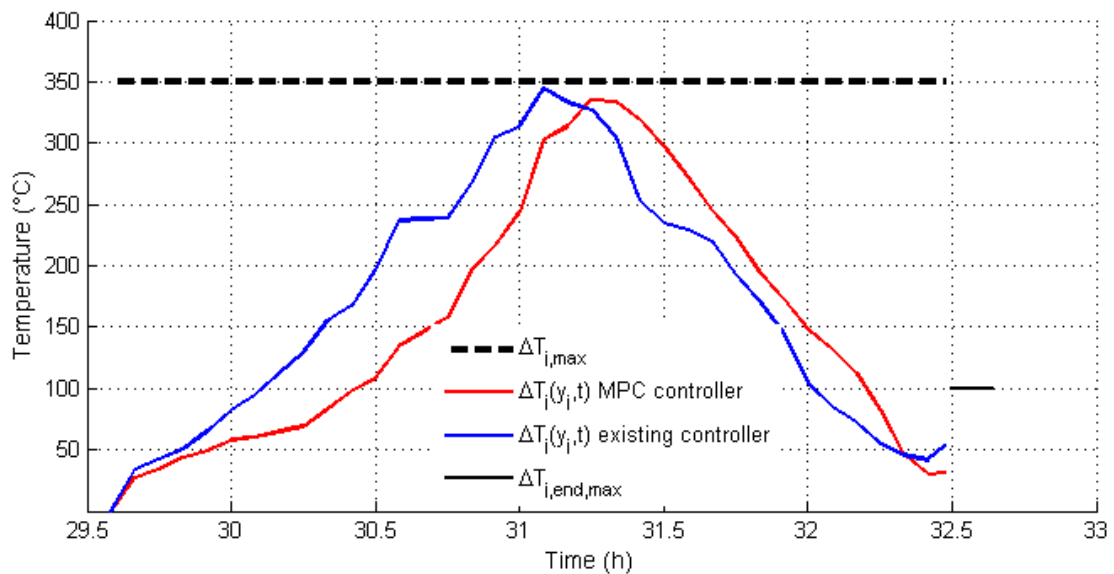
Figure 6.54: Temperature gradient of slab j = 400
