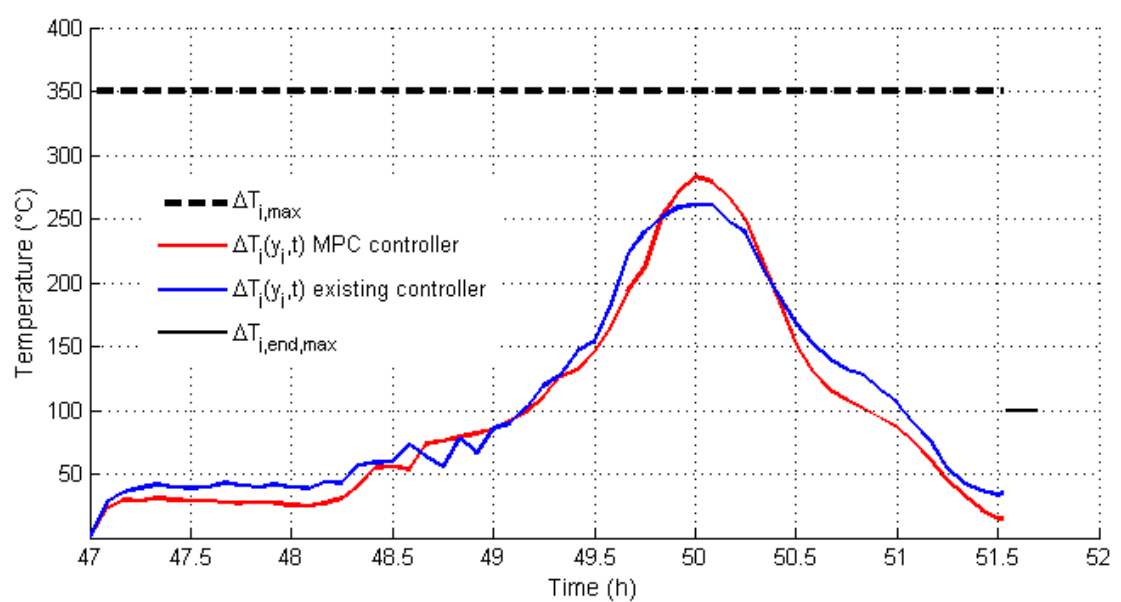
Figure 6.60: Temperature gradient of slab j = 641
