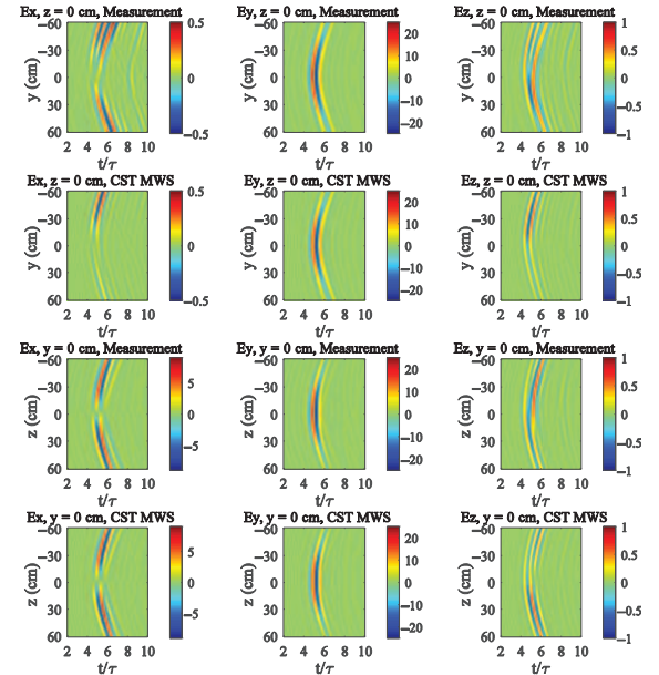
Fig. 14. NFN results at x = 40 \text{ cm} compared with the CST MWS results at the plane cuts y = 0 and z = 0 . NF data ( E_y and E_z ) have been measured at x_{\text{meas}} = 10 \text{ cm} from the AUT and transformed to reach the planar surface x = 40 \text{ cm} . The comparison comprises E_x , E_y , and E_z transient field components.
