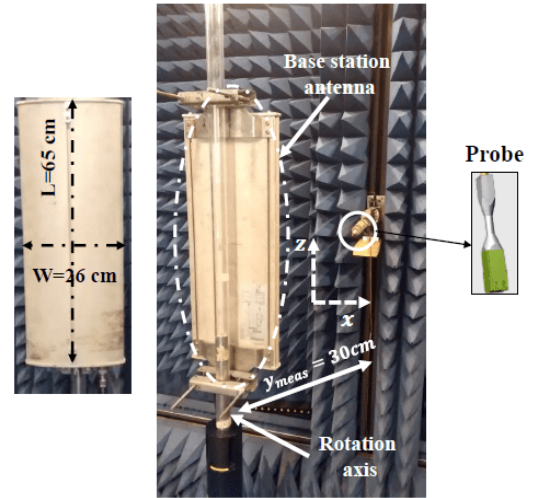
Fig. 14. Base station antenna measured in the planar NF facility.
