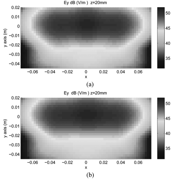
Fig. 7. The aperture field E_y (dB V/m) at the plane z = 0.02\text{m} ( 0.4\lambda ) from the AUT: (a) Resulted from the FEM simulation software. (b) Produced by the equivalent model associated to \Delta x = \Delta y = 0.25\lambda .
