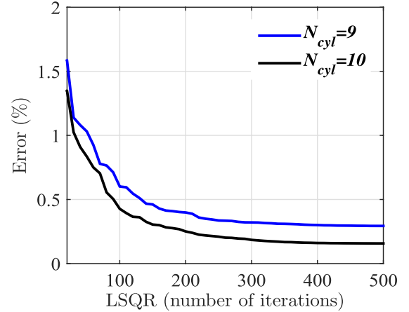
Fig. 3. Error function versus the number of LSQR iterations and the used number of cylindrical modes N_{cyl} .
