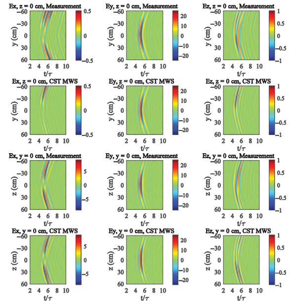
Fig. 14. NFN results at x = 40 cm compared with the CST MWS results at the plane cuts y = 0 and z = 0 . NF data ( E_y and E_z ) have been measured at x_{\text{meas}} = 10 cm from the AUT and transformed to reach the planar surface x = 40 cm. The comparison comprises E_x , E_y , and E_z transient field components.
