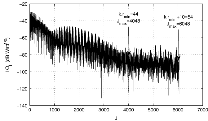
Fig. 7. Magnitude of the AUT transmission coefficients calculated using the measurement data collected over the spherical surface R_{\text{meas}} = 1.79 m, for 15 \leq \theta \leq 165^\circ and 105^\circ \leq \varphi \leq 255^\circ .
