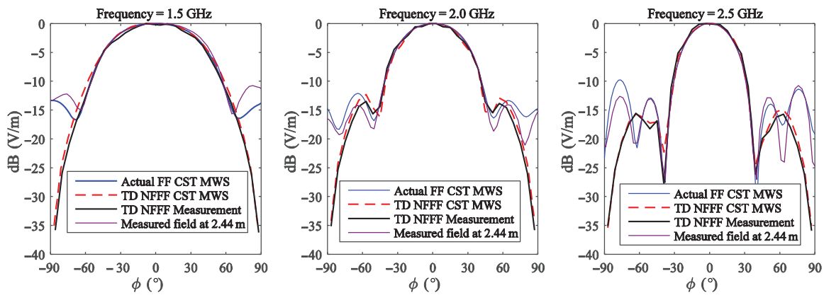
Fig. 15. Frequency domain results comparison. The FF issued from measured NF data ( x_{\text{meas}} = 10 cm) using the planar facility is compared with the CST MWS directly calculated FF for the frequencies 1.5, 2, and 2.5 GHz for the FF cut plane \theta = \pi/2 . The NFFF transformation results are Fourier transformed to calculate the frequency domain FF. The FF validity area is about \pm 48^\circ .
