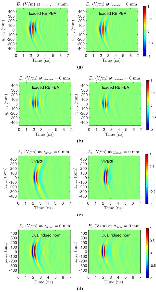
Fig. 11. Normalized transient radiated NFs at 100 mm in front of the antenna under test in the free space at plane cuts y_{meas} = 0 mm and z_{meas} = 0 mm for (a) loaded RB PBA, (b) loaded RB FBA, (c) Vivaldi antenna, and (d) dual ridged horn antenna.
