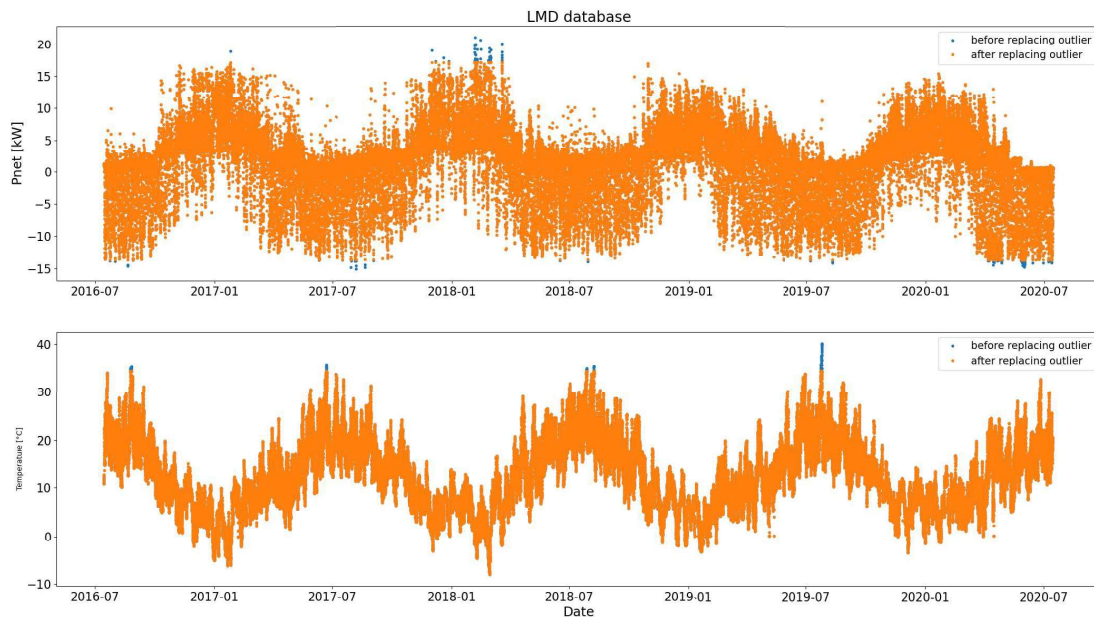
Figure 4.9: P_{net} and T_{out} outliers replacement ( \Delta t = 30\text{ min} )
