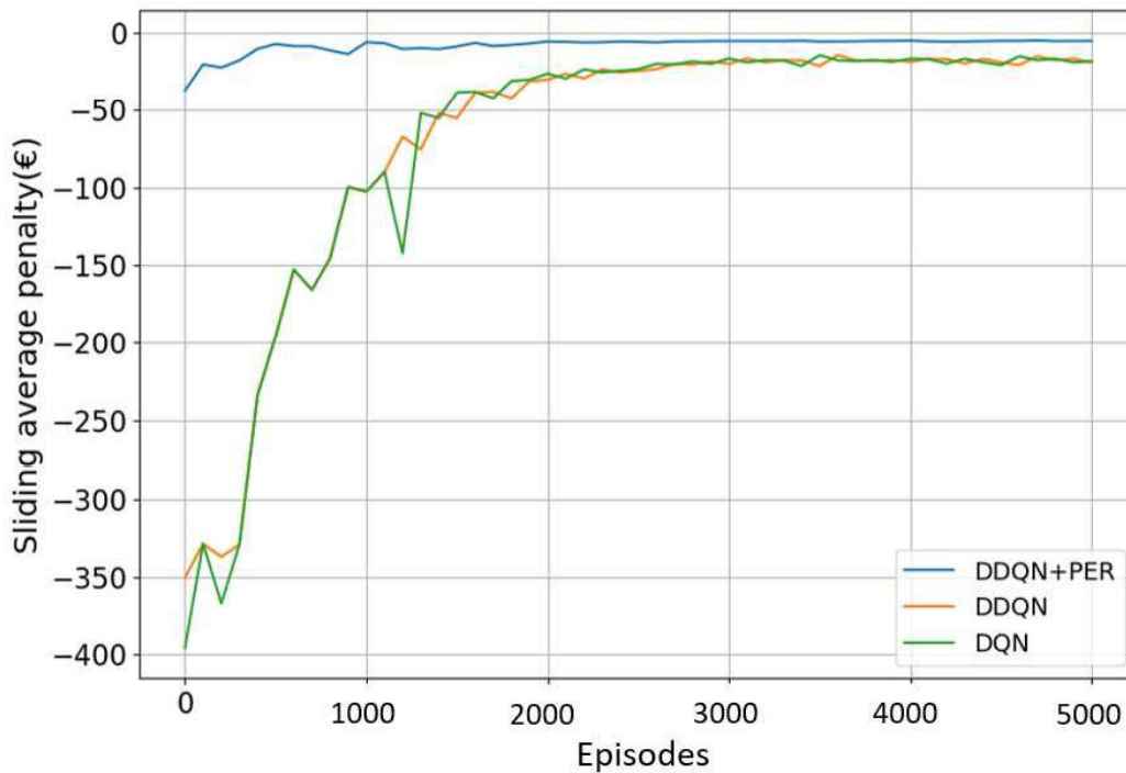
Figure 5.14: Learning curve for DQN, DDQN and DDQN+PER algorithm during autumn period
