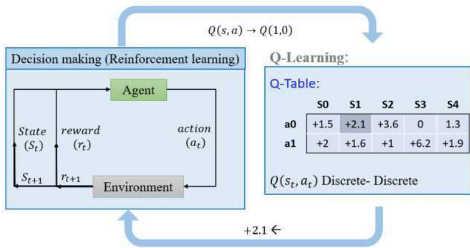
Figure 3.9: Q-learning mechanism
