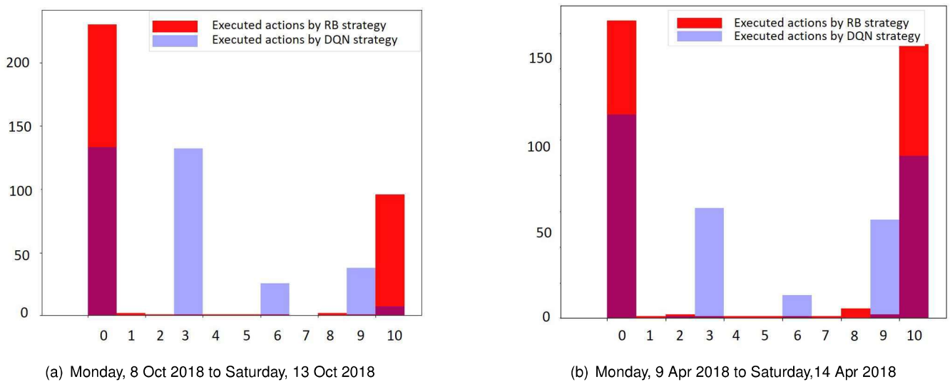
Figure 5.13: Histograms of the actions taken during each test phase
