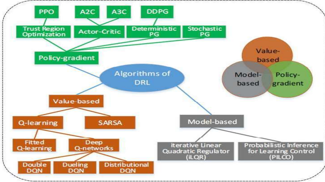
Figure 3.8: Main algorithms of DRL and their relationship[88]
